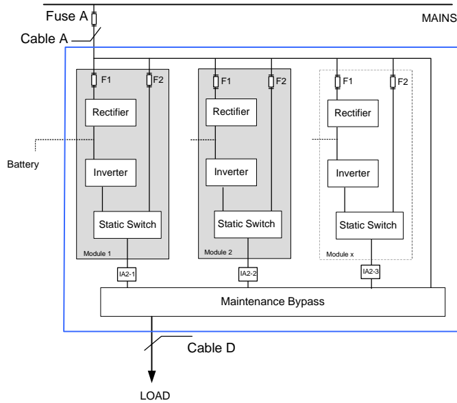
SINGLE INPUT FEED - STANDARD VERSION
