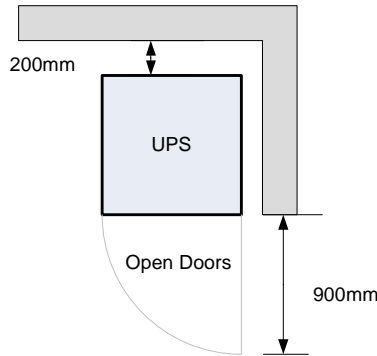
Figure 1: UPS space recommendation
