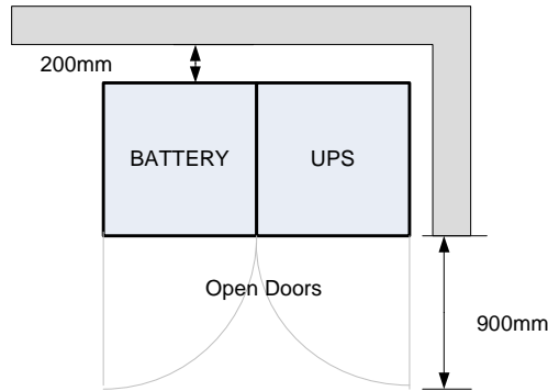
Figure 2: UPS + Battery space recommendation
