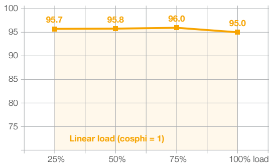
AC-AC efficiency (60–120)
