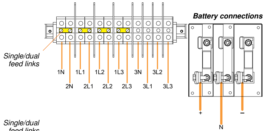
60kVA- 100kVA Power connections
