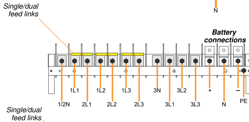
120kVA- 200kVA Power connections
