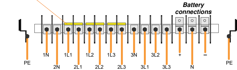
250kVA- 300kVA Power connections
